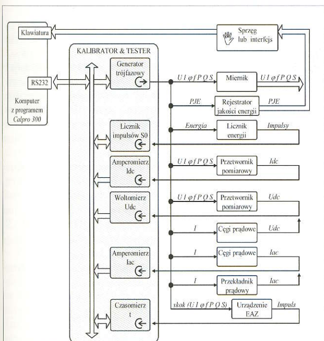
Rys. 3. System z kalibratorem / testerem Fig. 3. System with calibrator / tester
